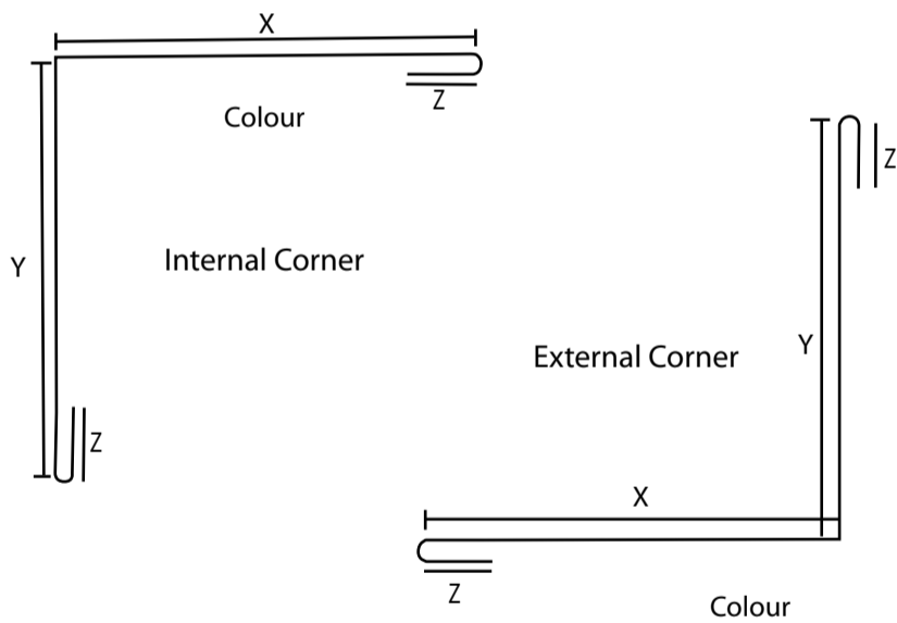
Corner Flashings
