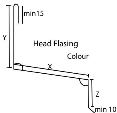
Window Flashings
