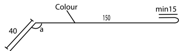
Gutter Flashings
